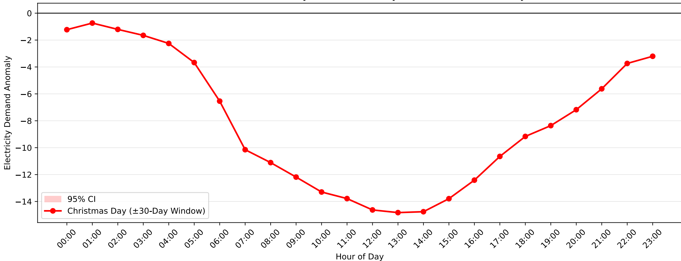
Marrickville Demand Anomaly: Christmas Day (2004–2005, \pm 30 -Day Window)
